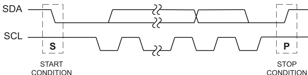
Figure 7. Bit Transfer
