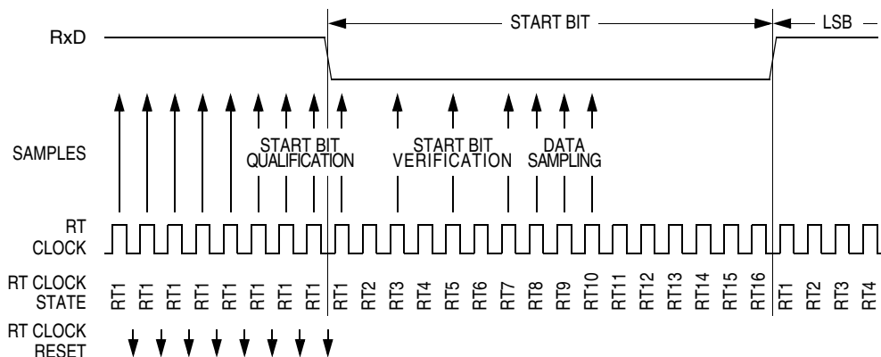
Figure 14-7. Receiver Data Sampling
