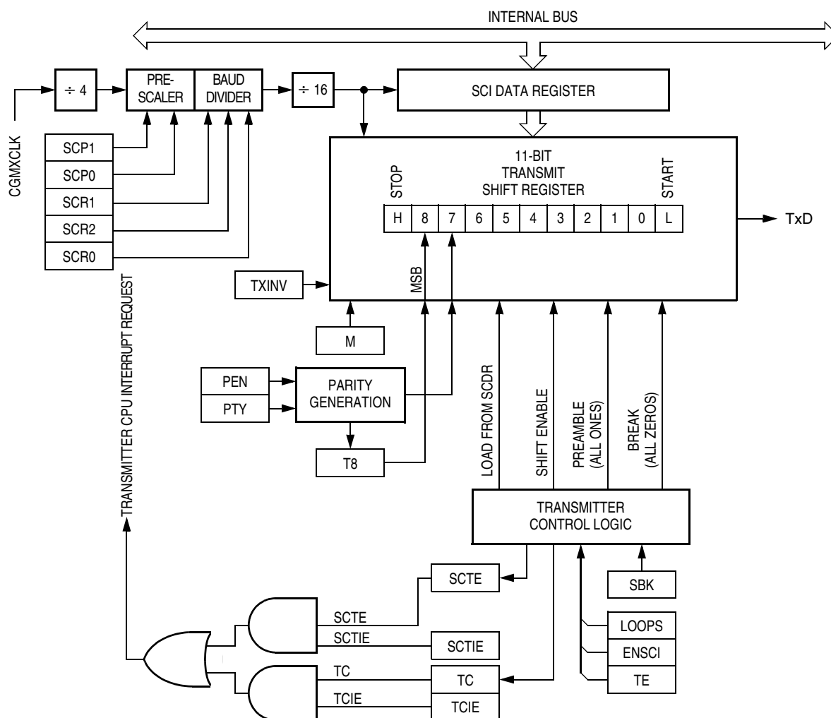
Figure 14-5. SCI Transmitter
