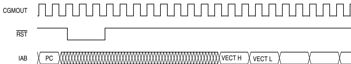
Figure 15-5. External Reset Timing
