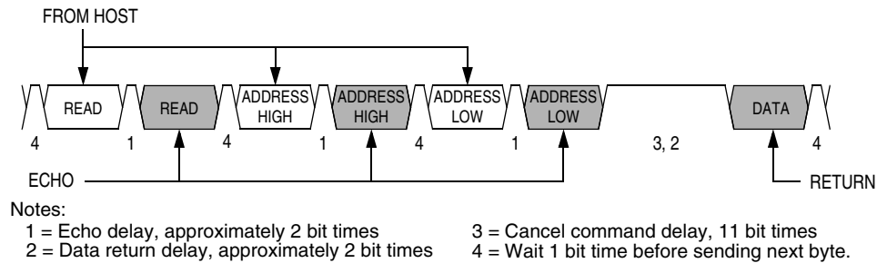
Figure 19-11. Read Transaction
