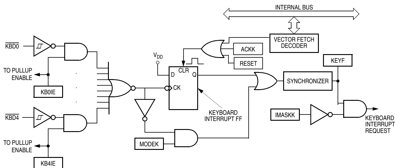
Figure 8-2. Keyboard Module Block Diagram
