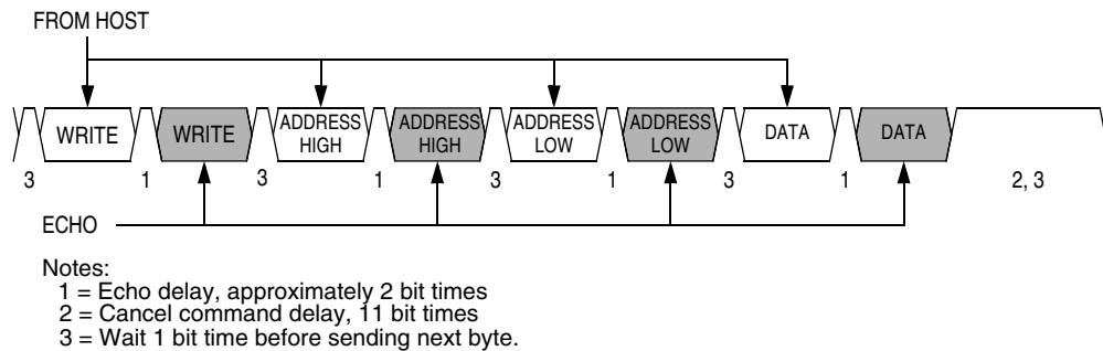
Figure 19-12. Write Transaction
