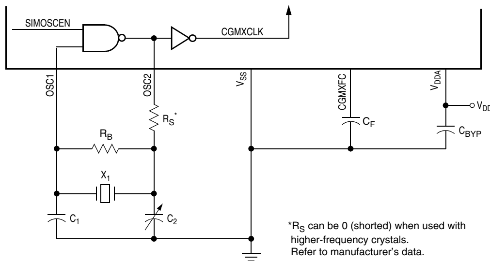
Figure 4-3. CGM External Connections
