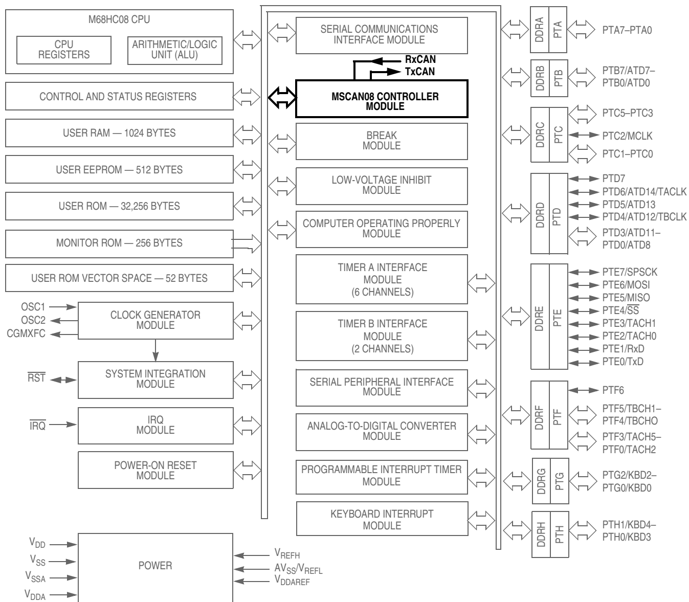
Figure 11-1. Block Diagram Highlighting MSCAN08 Block and Pins
