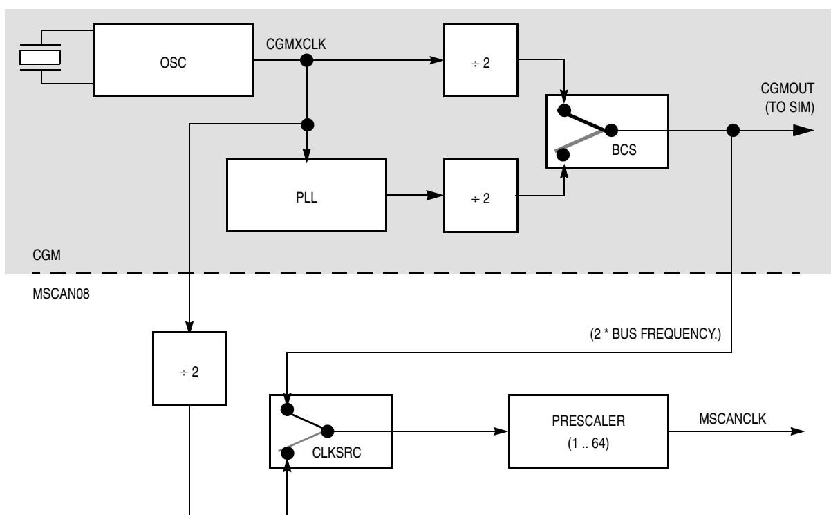
Figure 11-8. Clocking Scheme
