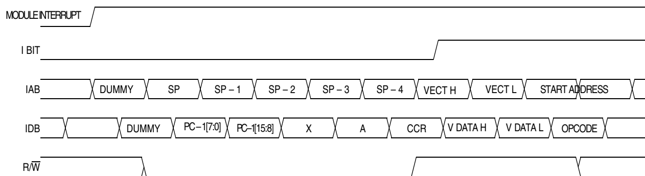
Figure 15-9. Interrupt Entry
