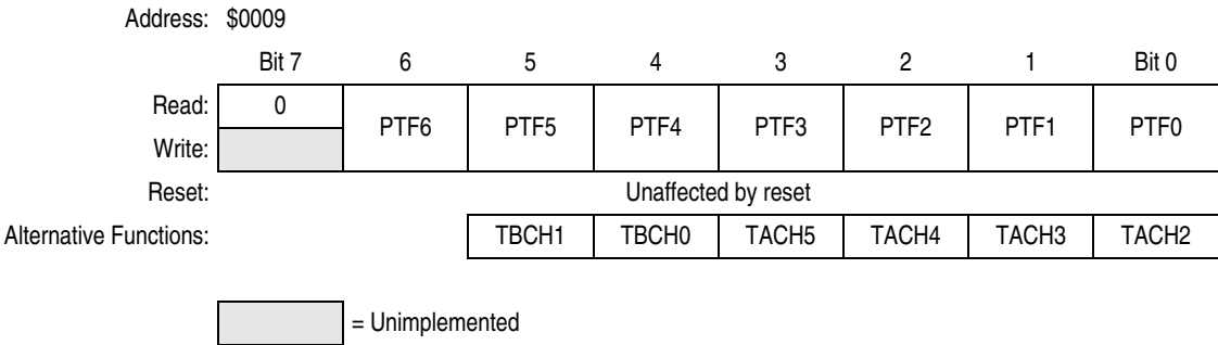
Figure 13-17. Port F Data Register (PTF)
