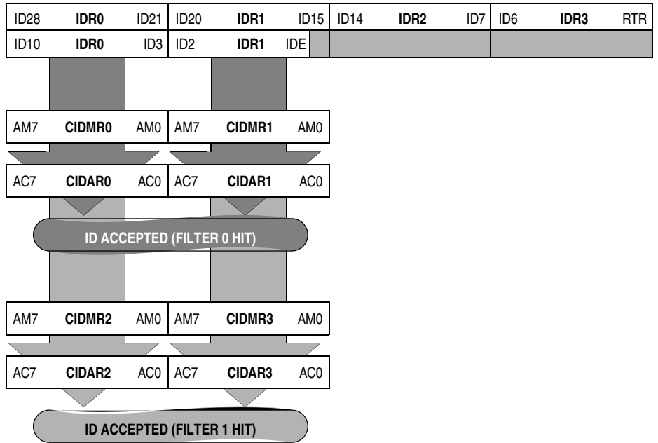
Figure 24-4. Dual 16-Bit Maskable Acceptance Filters
