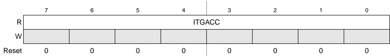
Figure 10-9. Integration Accumulator Register Low (ITGACC)
