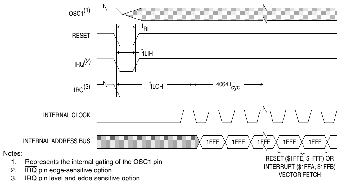
Figure 6-2. Stop Recovery Timing Diagram
