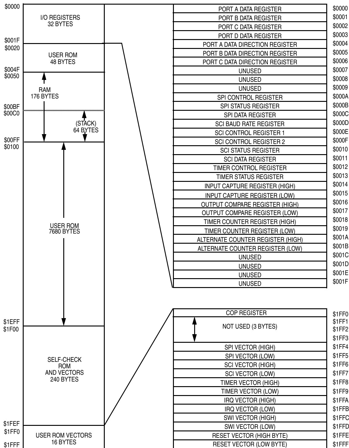
Figure 2-1. Memory Map
