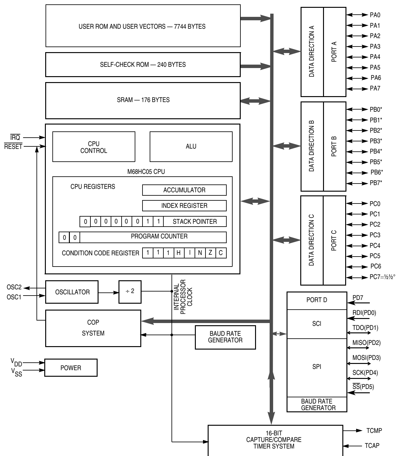
Figure 1-1. Block Diagram
