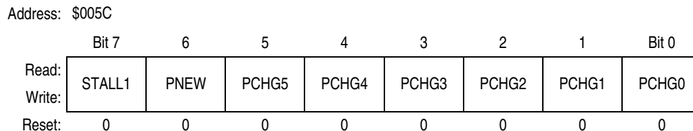
Figure 9-11. USB HUB Control Register 1 (HCR1)
