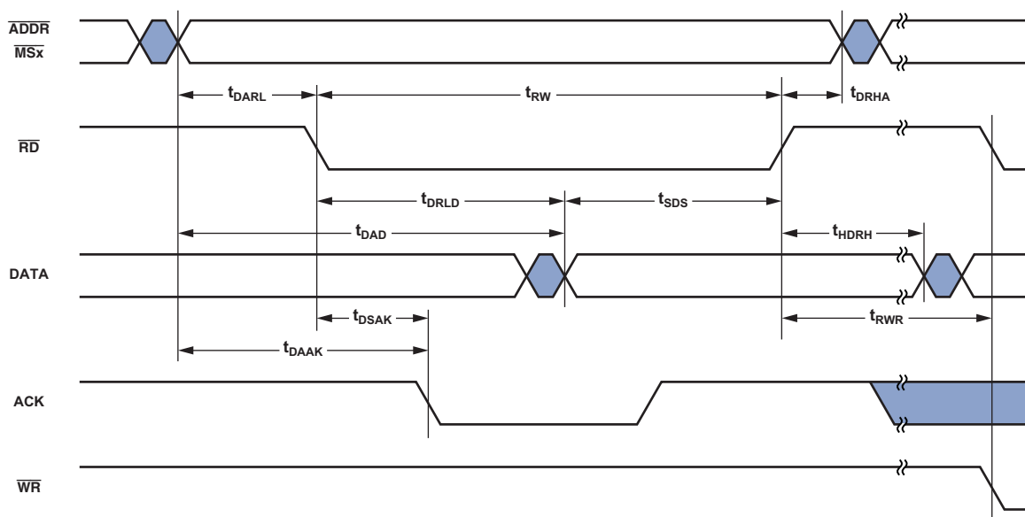
Figure 19. Memory Read
