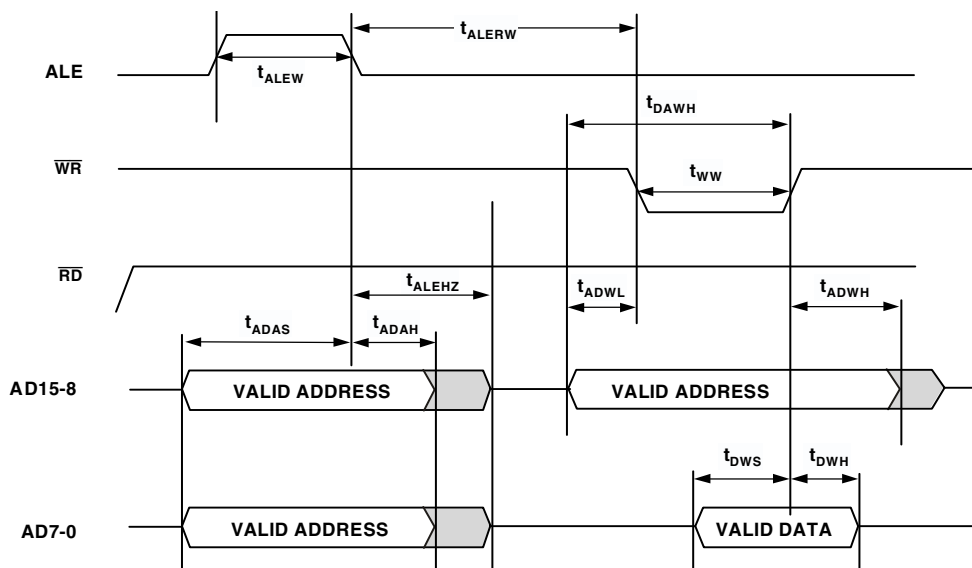
Figure 18. 8-Bit Memory Write Cycle
