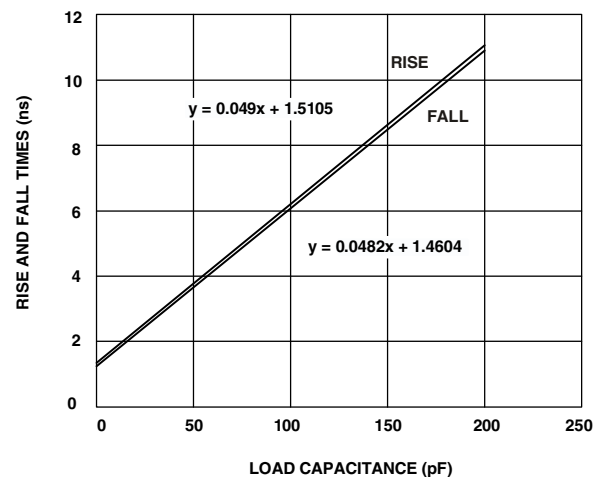
Figure 31. Typical Output Rise/Fall Time (20% to 80%, V_{DDEXT} = \text{Min} )
