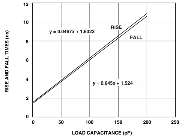
Figure 30. Typical Output Rise Time (20% to 80%, V_{DDEXT} = \text{Max} )
