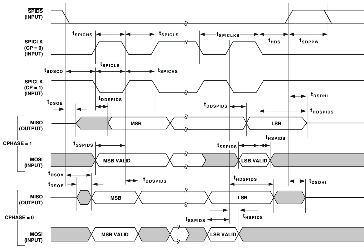
Figure 25. SPI Interface Protocol—Slave
