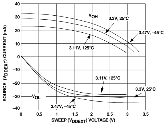
Figure 27. Typical Drive
