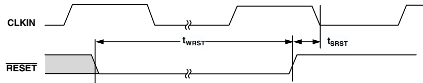
Figure 8. Reset
