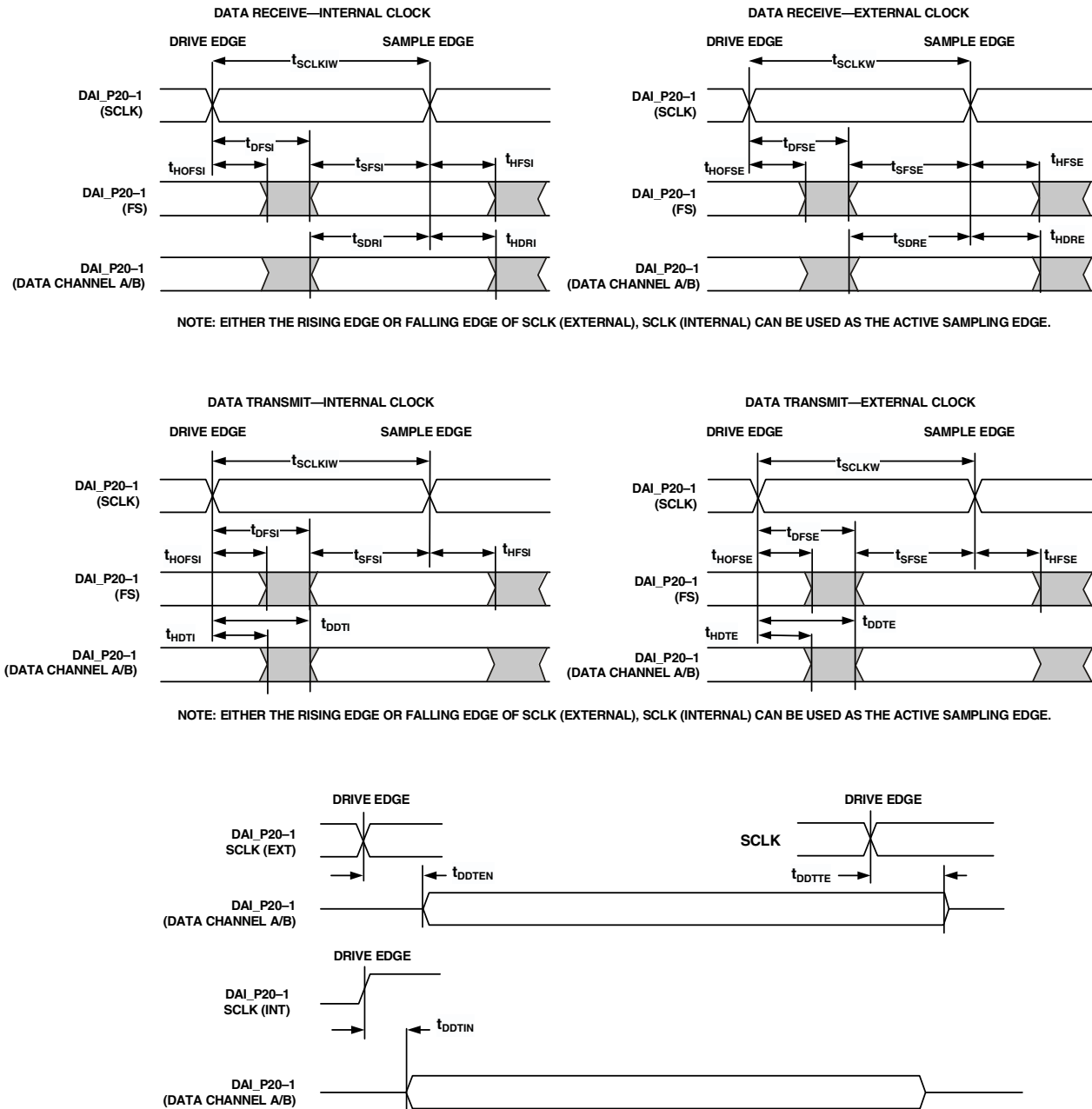
Figure 21. Serial Ports
