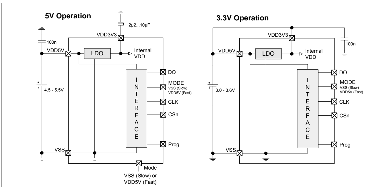
Figure 5 Connections for 5V / 3.3V Supply Voltages
