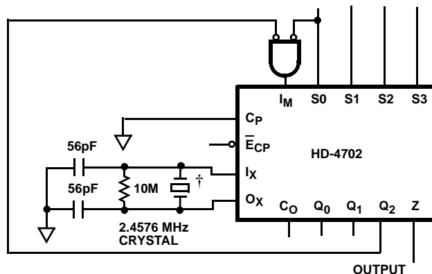
FIGURE 3. 19200 BAUD OPERATION
