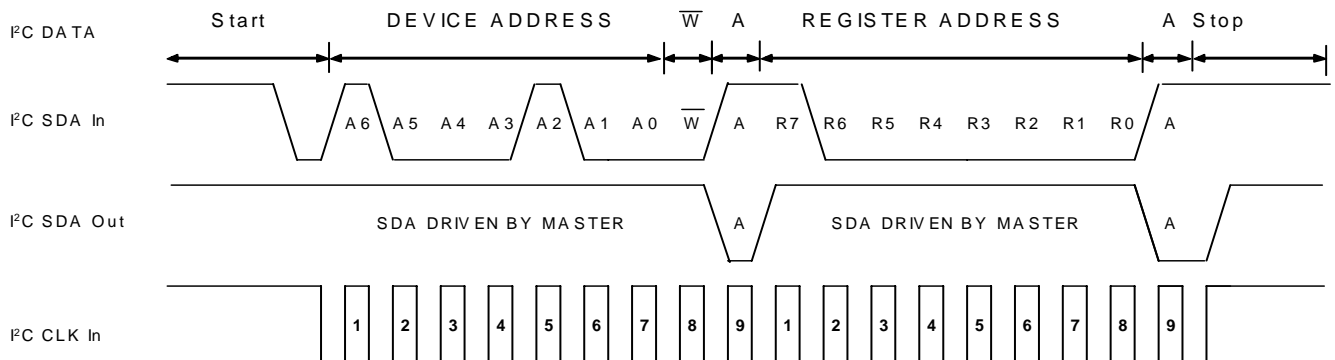
FIGURE 3. I²C SYNC_I²C TIMING DIAGRAM SAMPLE
