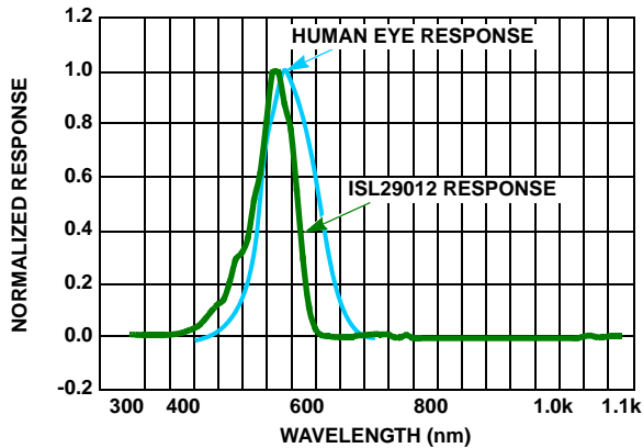
FIGURE 7. SPECTRAL RESPONSE
