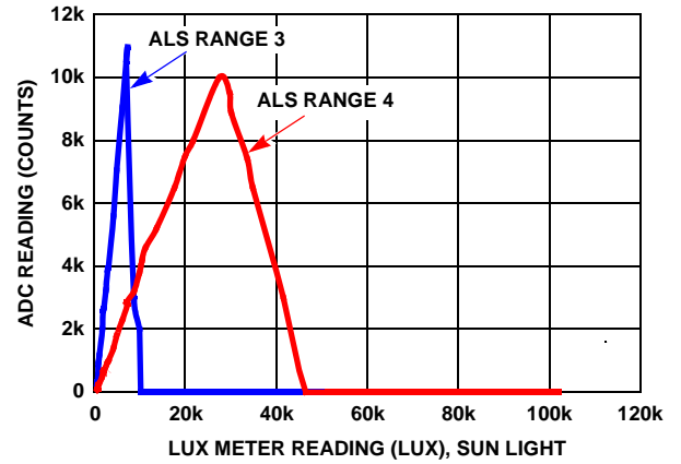
FIGURE 18. SATURATION CHARACTERISTICS
