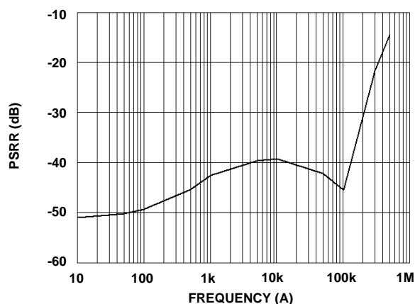
FIGURE 10. LDO1 POWER SUPPLY REJECTION ( I_{OUT1} = 100mA , C_{OUT} = 10\mu F MLCC)
