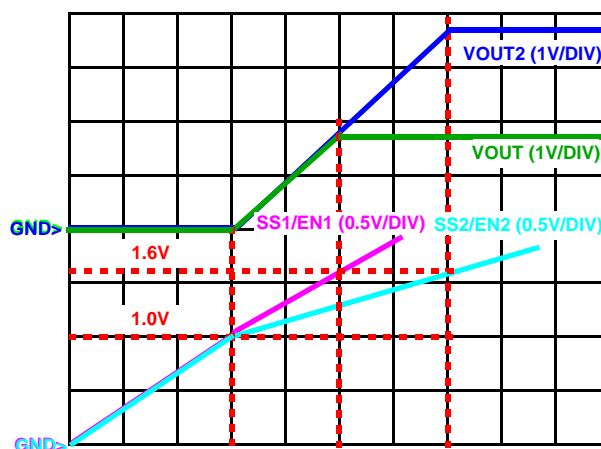
FIGURE 6. VOLTAGE TRACKING
