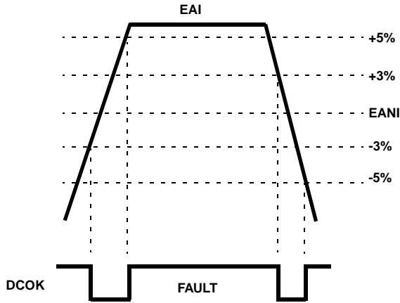
FIGURE 11. UNDERVOLTAGE-OVERVOLTAGE WINDOW
