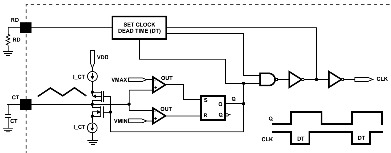
FIGURE 1. SIMPLIFIED CLOCK GENERATOR CIRCUIT
