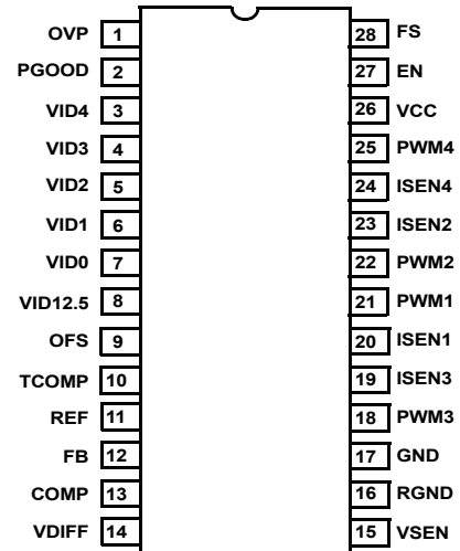
28 LEAD SOIC TOP VIEW
