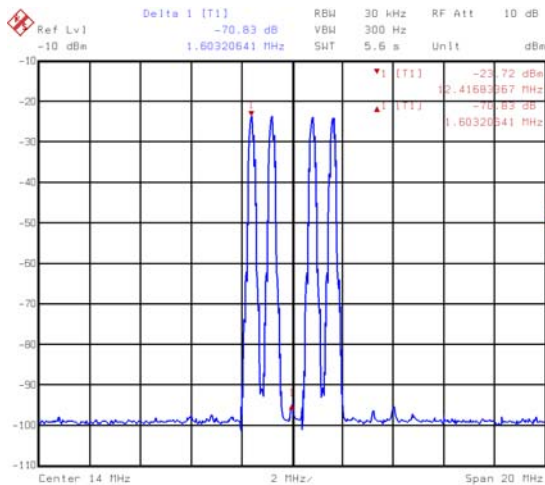
FIGURE 5. FOUR EDGE CARRIERS AT 12.4MHz TO 15.6MHz, 800kHz SPACING, 78MSPS (71dBc - 20MHz WINDOW)
