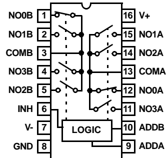
ISL84052 (16 LD SOIC, QSOP, TSSOP) TOP VIEW
