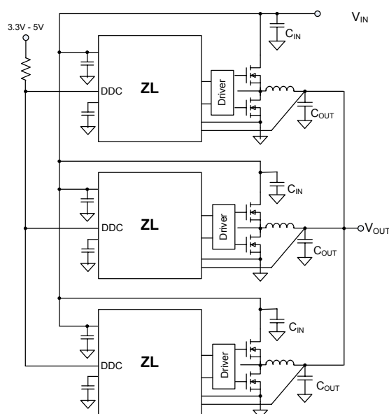
Figure 19. Current Sharing Group
