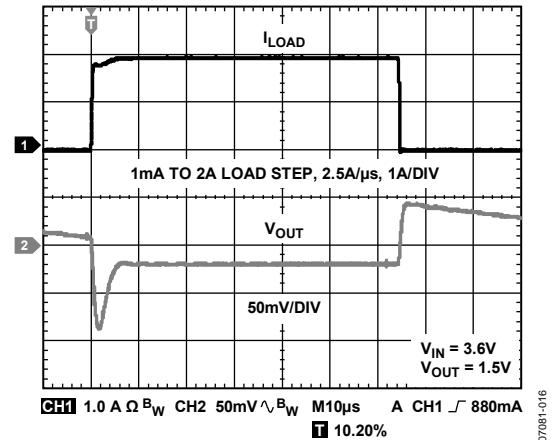
Figure 16. Load Transient Response, C_{IN} = 22\text{ }\mu\text{F} , C_{OUT} = 22\text{ }\mu\text{F}
