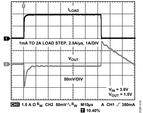
Figure 15. Load Transient Response, C_{IN} = 4.7\text{ }\mu\text{F} , C_{OUT} = 4.7\text{ }\mu\text{F}
