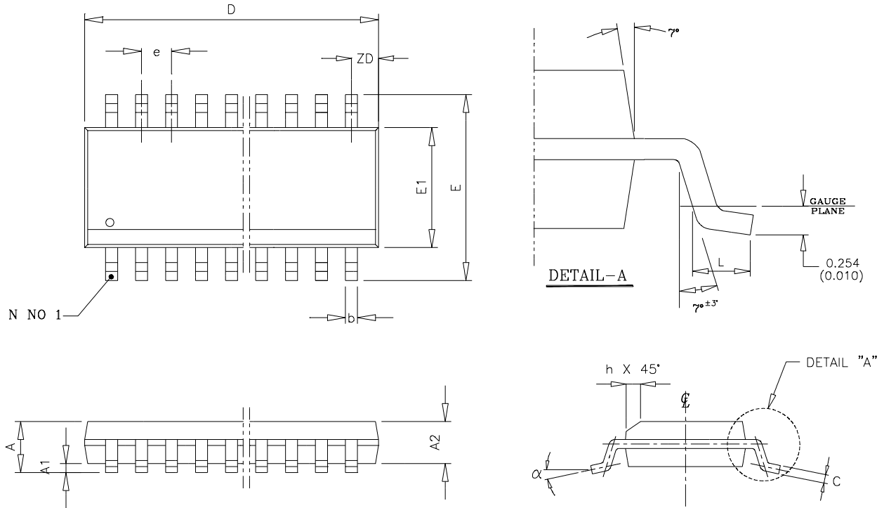
Figure 21. QSOP-24 Package
