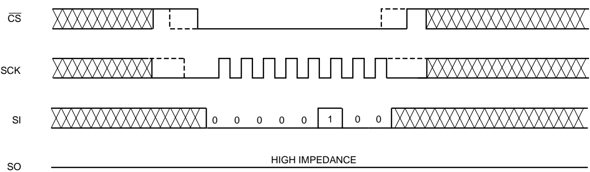
Figure 5. WRDI Timing
