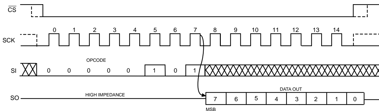
Figure 11. RDSR Timing
