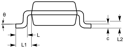
END VIEW
