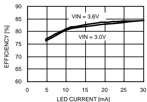
Efficiency – Three LEDs
