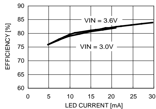
Efficiency – Four LEDs
