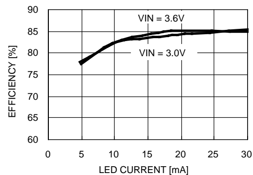
Efficiency – Two LEDs
