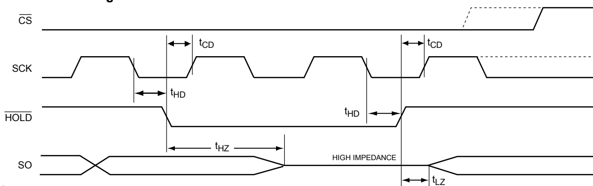
Figure 2. \overline{\text{HOLD}} Timing
