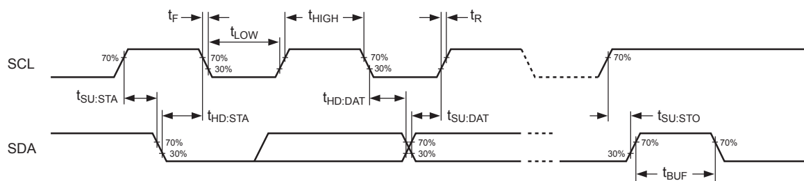
Figure 4. Bus Timing
