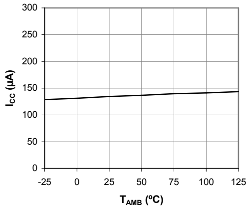
TS Active Current (I 2 C-bus idle)
