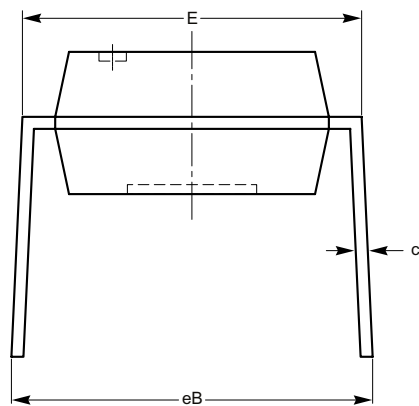
END VIEW
