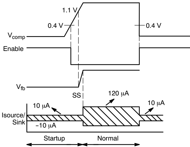
Figure 12. Soft-Start Implementation
