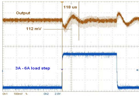
Figure 23. Transient Response ( V_{in} = 13.2\text{ V} , V_{out} = 3.3\text{ V} , I_{out} = 3\text{ A} to 6\text{ A} Step) Output Capacitors: 2x MLCC 100\text{ }\mu\text{F} and 820\text{ }\mu\text{F} OS-CON
