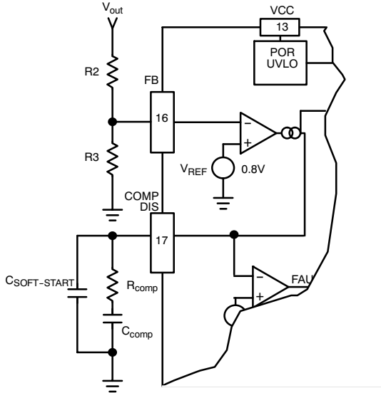
Figure 17. FB circuit
