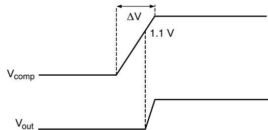
Figure 15. Soft-Start
