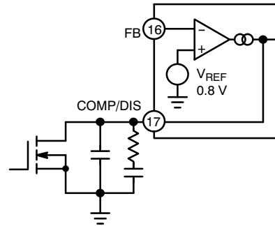
Figure 11. Disable Circuit
