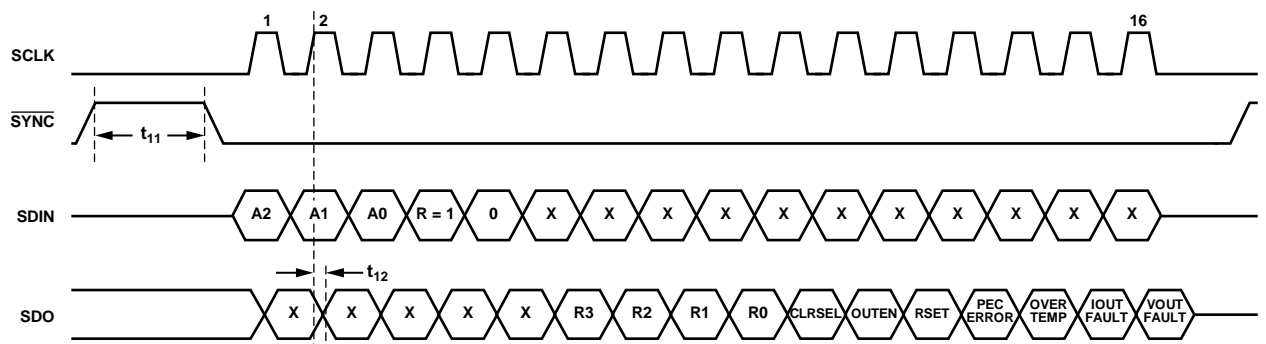
Figure 3. Readback Mode Timing Diagram
