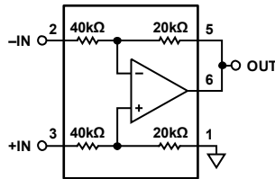
Figure 48. Difference Amplifier, Gain = 1/2
