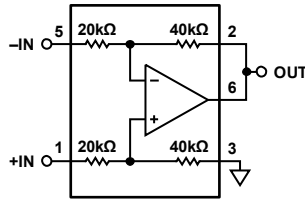
Figure 49. Difference Amplifier, Gain = 2
