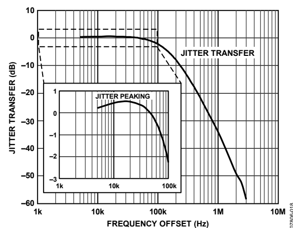
Figure 5. Jitter Transfer and Jitter Peaking
