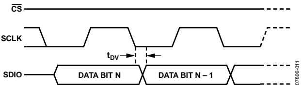
Figure 25. Timing Diagram for Serial Control Port Register Read
