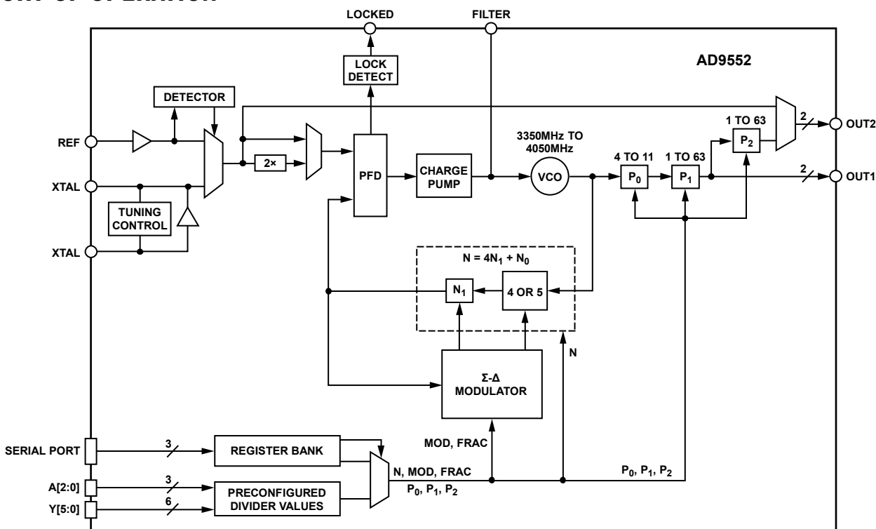
Figure 17. Detailed Block Diagram
