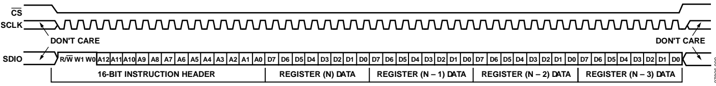
Figure 23. Serial Control Port Read—MSB First, 16-Bit Instruction, Four Bytes Data
