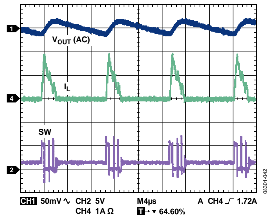
Figure 32. PFM Mode
