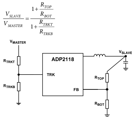
Figure 42. Voltage Tracking
