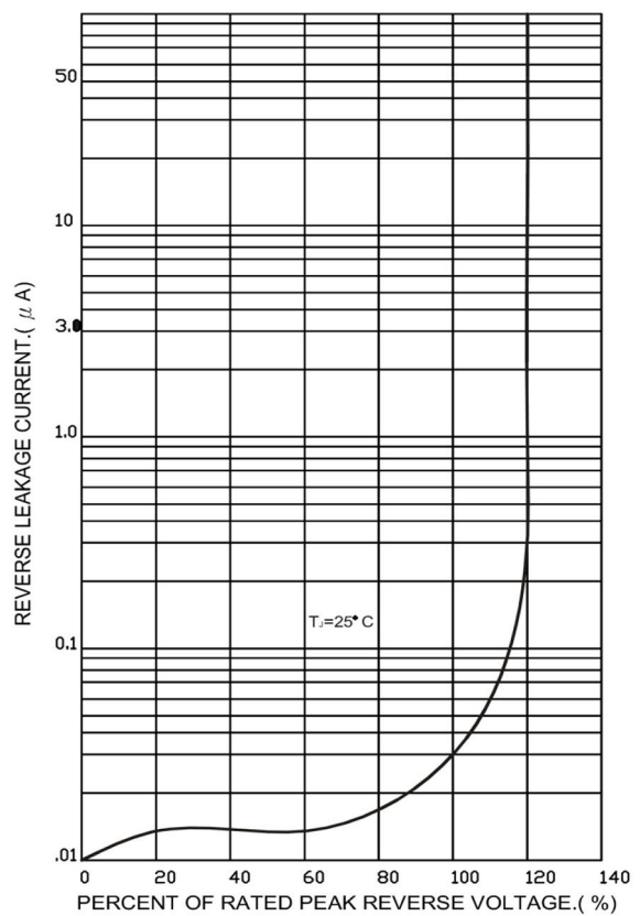
FIG.4-TYPICAL REVERSE CHARACTERISTICS
