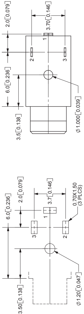
PCB LAYOUT TOP VIEW
