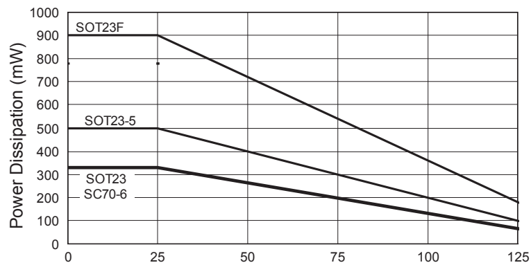
Power Dissipation Derating
