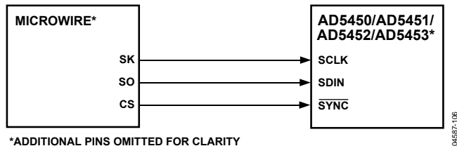
Figure 59. MICROWIRE-to-AD5450/AD5451/AD5452/AD5453 Interface
