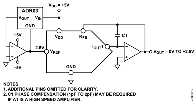
Figure 46. Positive Output Voltage with Minimum Components
