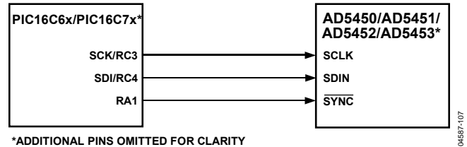
Figure 60. PIC16C6x/7x-to-AD5450/AD5451/AD5452/AD5453 Interface
