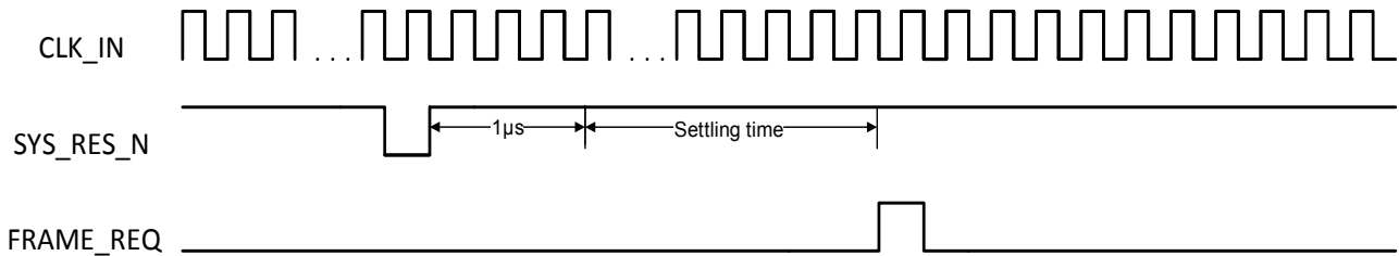
FIGURE 9: RESET SEQUENCE
