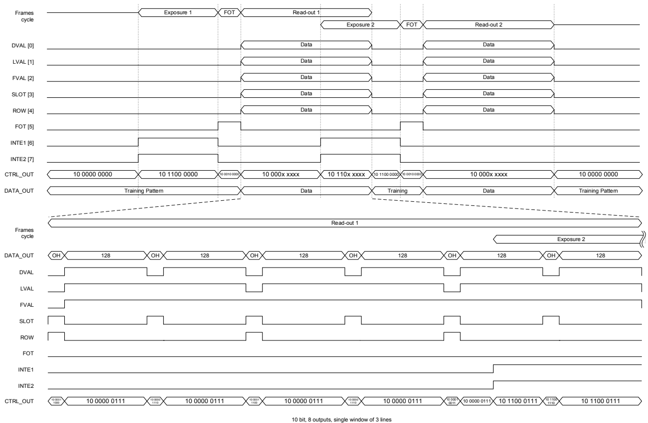
FIGURE 31: DVAL, LVAL AND FVAL TIMING IN 8 OUTPUT MODE
