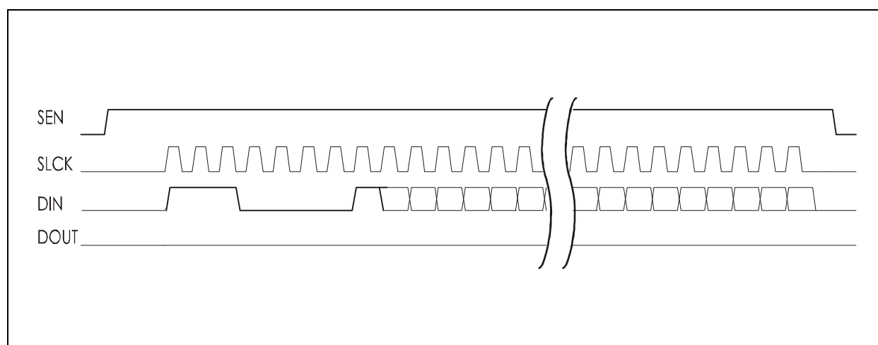
Figure 38: SPI Write FIFO Command
