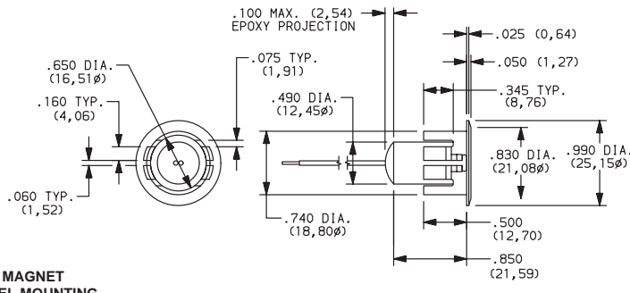
MAGNET
