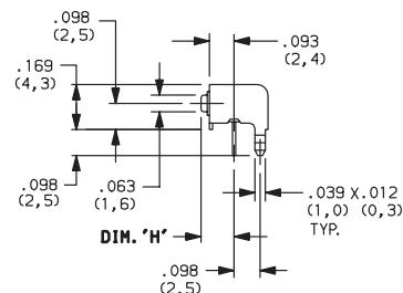
PTS635VL31 SPST
