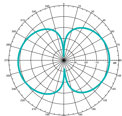
2.5GHz 1.59034dBi
