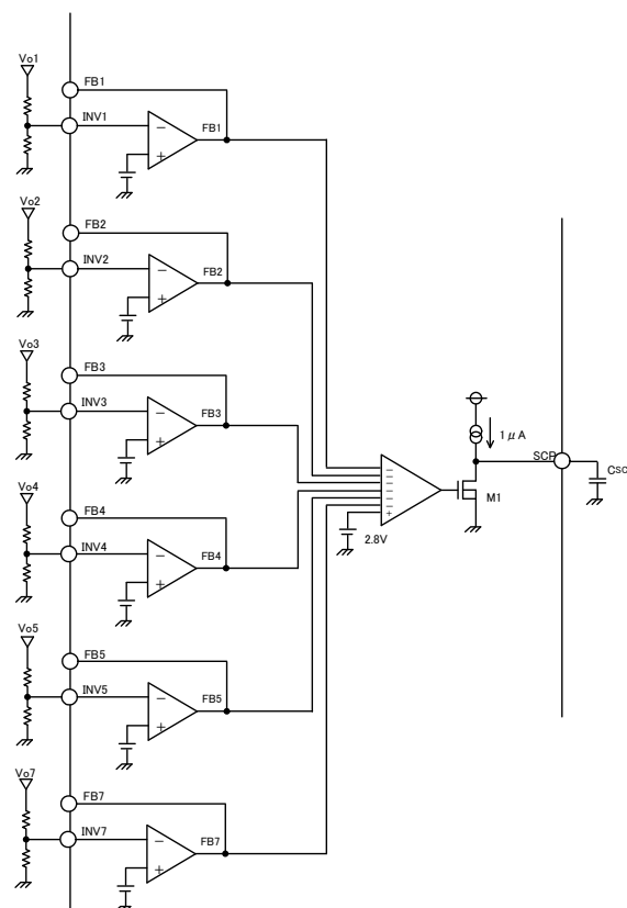
Fig. 8 Block diagram of short circuit protection circuit.
