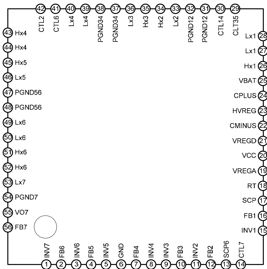
Fig. 2 Pin Assignments
