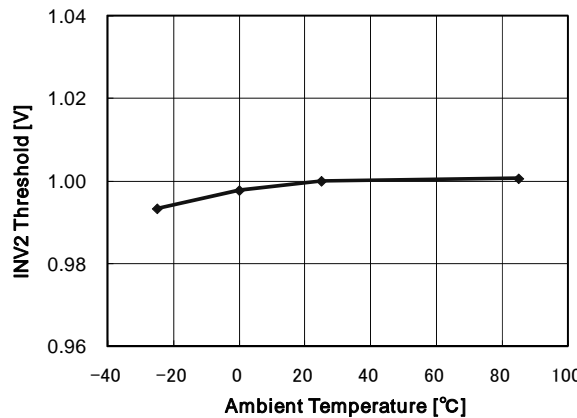
Fig. 15 CH2 ErrorAmp. INV threshold vs ambient temperature
