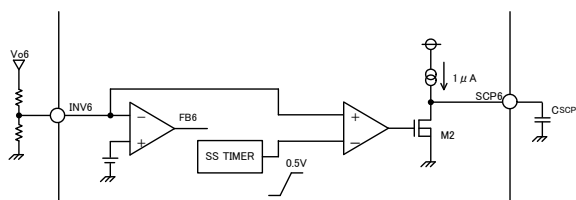
Fig. 9 Block diagram of short circuit protection6 circuit.
