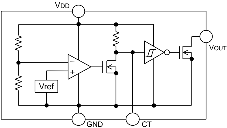
Fig.1 BD52xx Series
