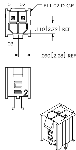
FIG 7 (IPL1-102-01-XXX-D-G SHOWN) (DIFFERENT AS SHOWN, OTHERWISE SAME AS FIG 1)
