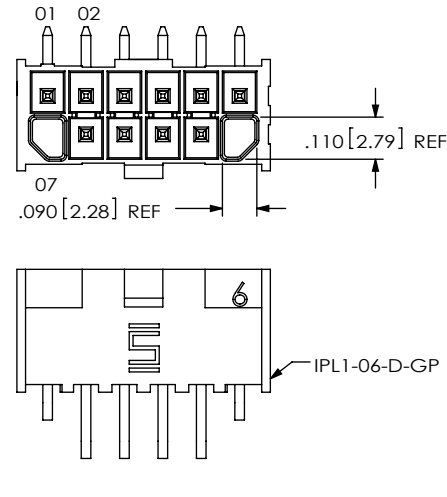
FIG 6 (IPL1-106-01-XXX-D-RA-G SHOWN) (DIFFERENT AS SHOWN, OTHERWISE SAME AS FIG 3)
