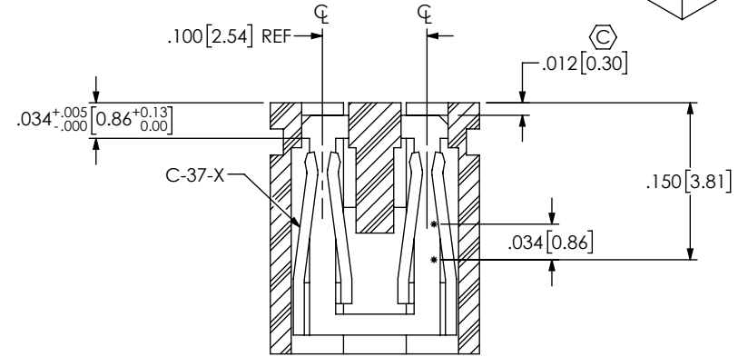
SECTION "A"-"A" SCALE 6:1
