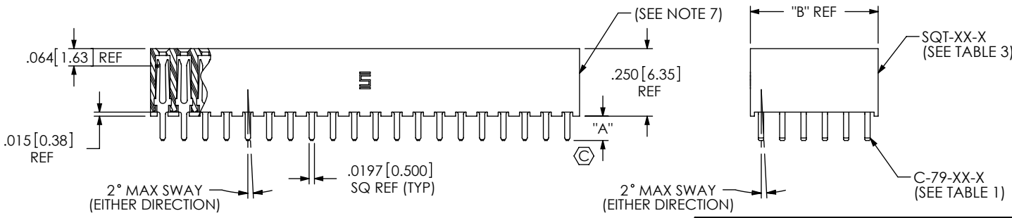
FIG 1 SQT-120-01-XX-6 SHOWN
