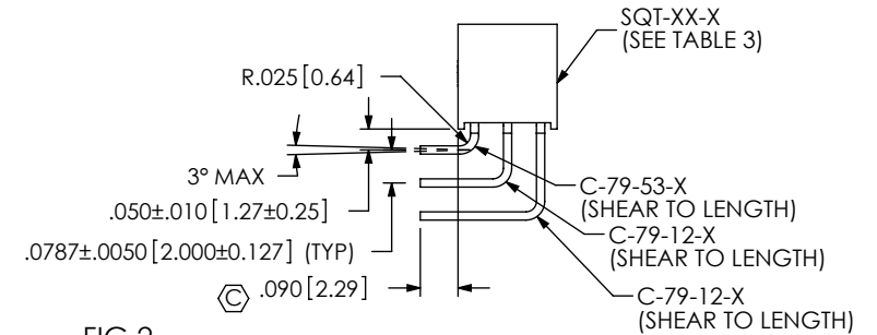
FIG 2 -RA: RIGHT ANGLE (LEAD STYLE -01-D,T)
