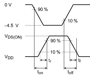
Fig. 5.3.2 Input Waveform/Output Waveform
