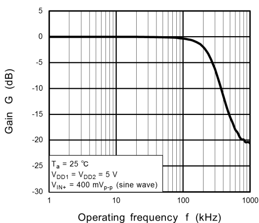
Fig. 12.11 G[\text{dB}] - f
