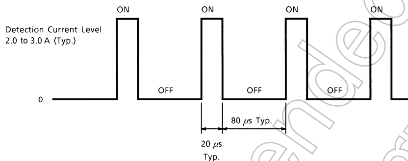
Figure 1 Basic Operation
