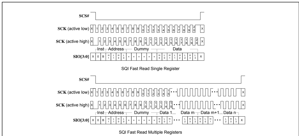
FIGURE 10-6: SQR FAST READ
