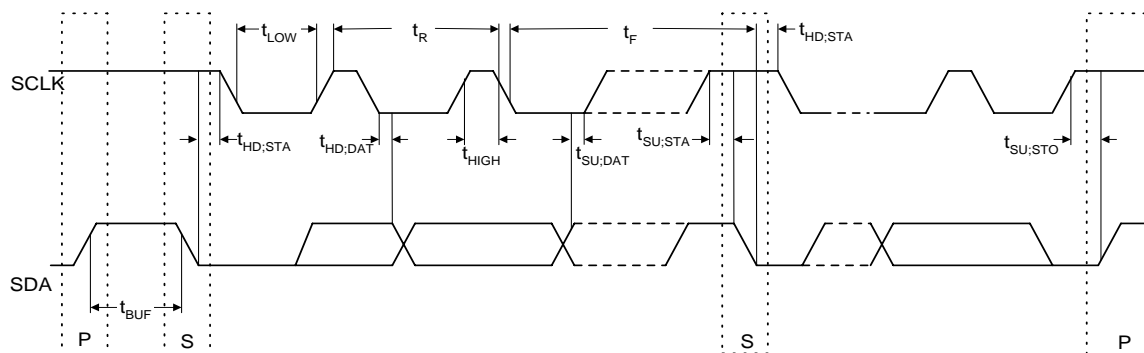
Figure 9.2 SMBus Timing
